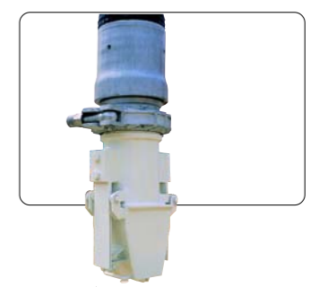
混凝土防离析装置 防止混凝土离析,提高工程质量。 避免待料堵管,延长输送管寿命。 The device to avoid concrete segregation Avoid the concrete segregation, raise working efficiency, prevent from blocking while waiting for materials, and prolong the life of bend pipe.
