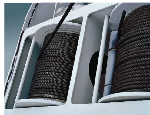
● 简单而巧妙的双重防乱绳装置 ● Simple and skillful double preventing rope installation
